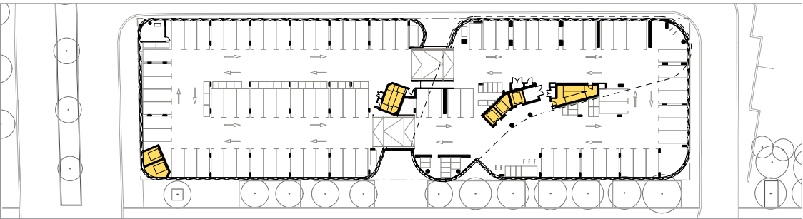
Level 4 plan (car park)
