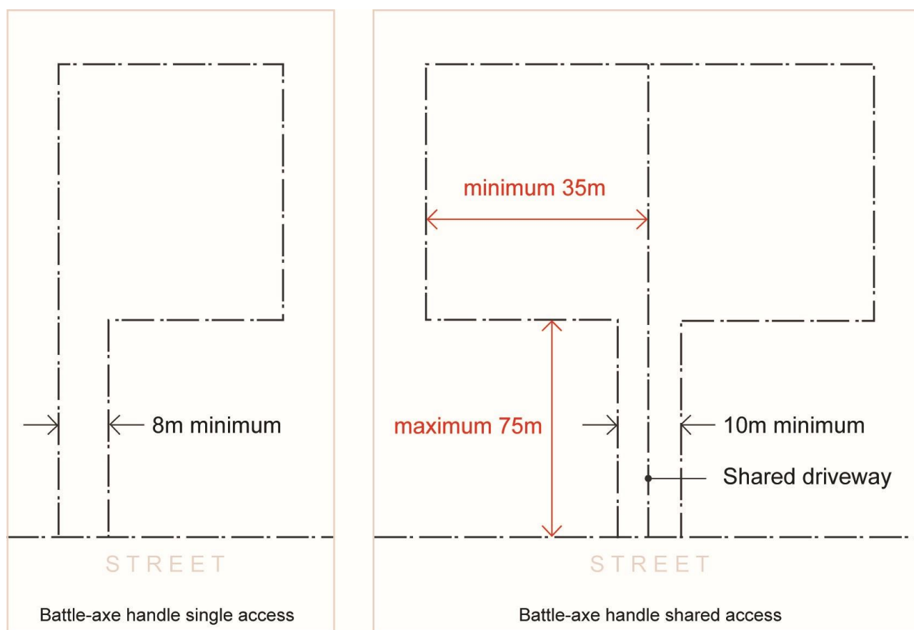
Figure 6-1. Battle axe lot dimensions
