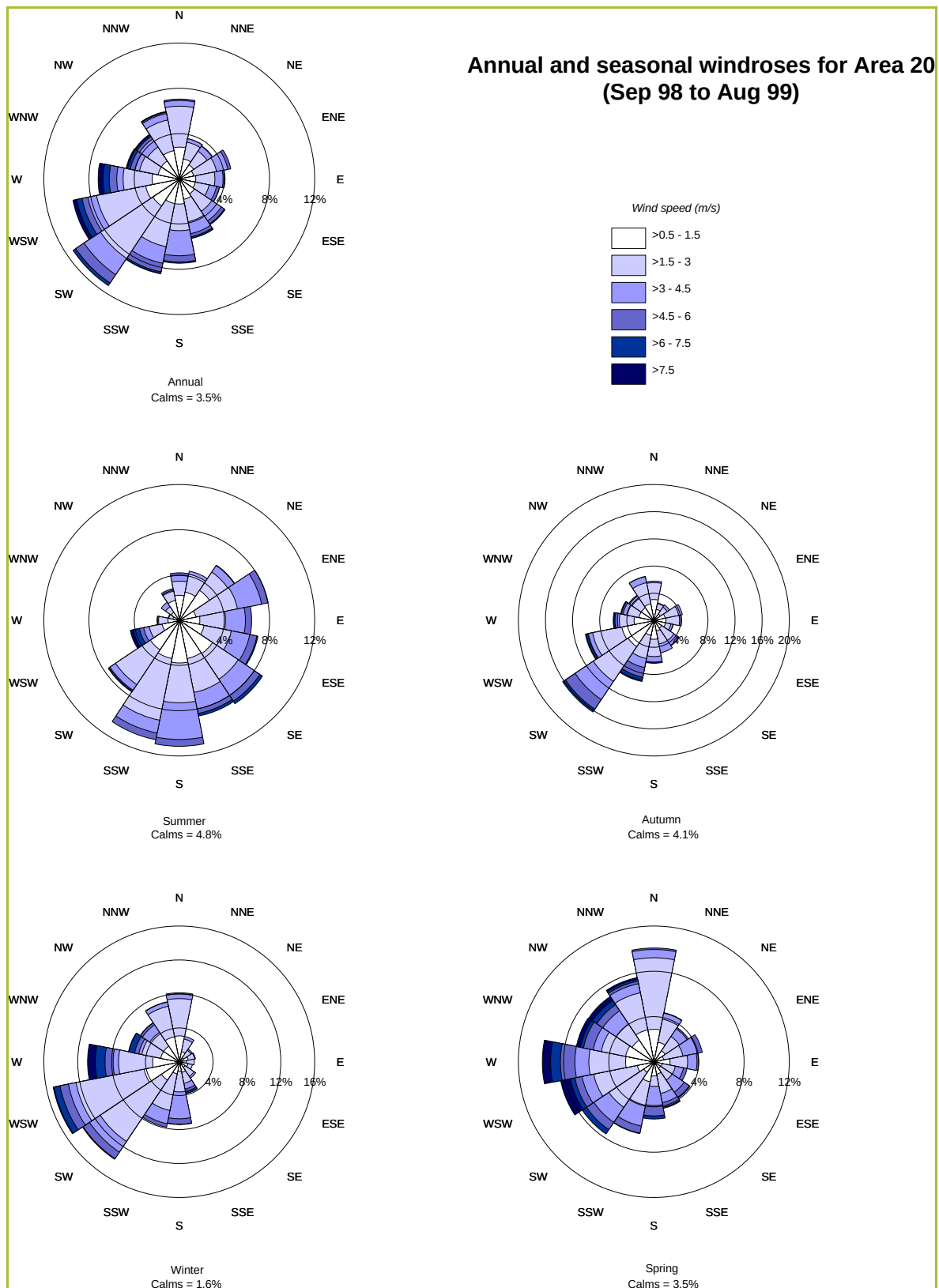
Figure B.1: Annual and seasonal windroses
