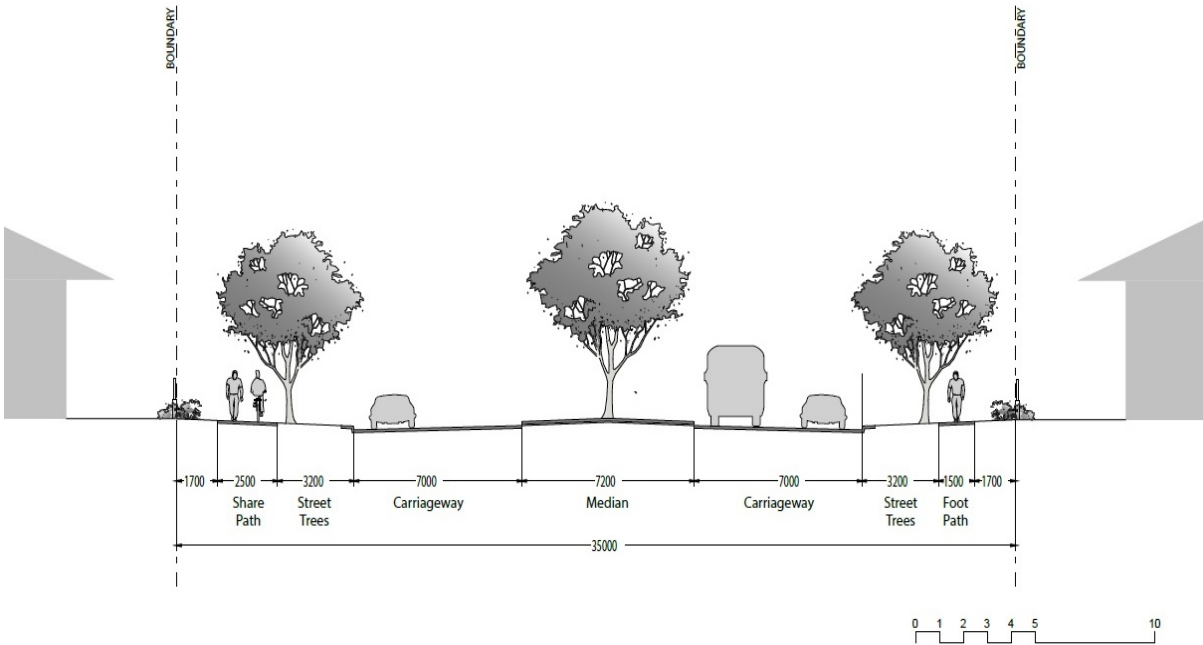
Figure 4-3 Sub Arterial
