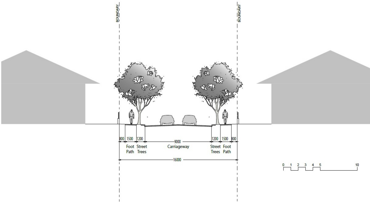
Figure 4-5 Local Street
