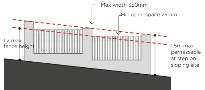
Figure 3-47 On sloping sites fences and walls should be stepped so that no part of the fence is higher than 1.5m above natural ground level
