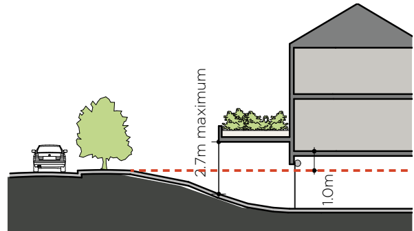
Figure 3-51 Reduce visual impact of basement entries by reducing the scale of the garage opening
