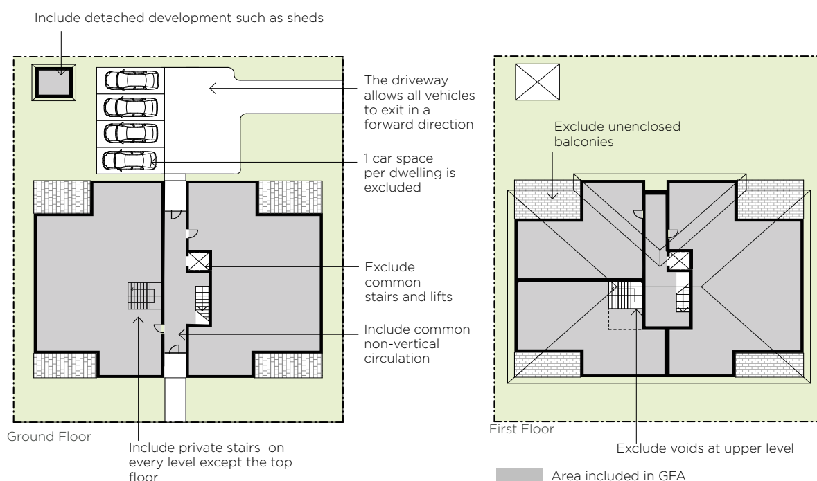
Figure 3-36 Calculating gross floor area.
