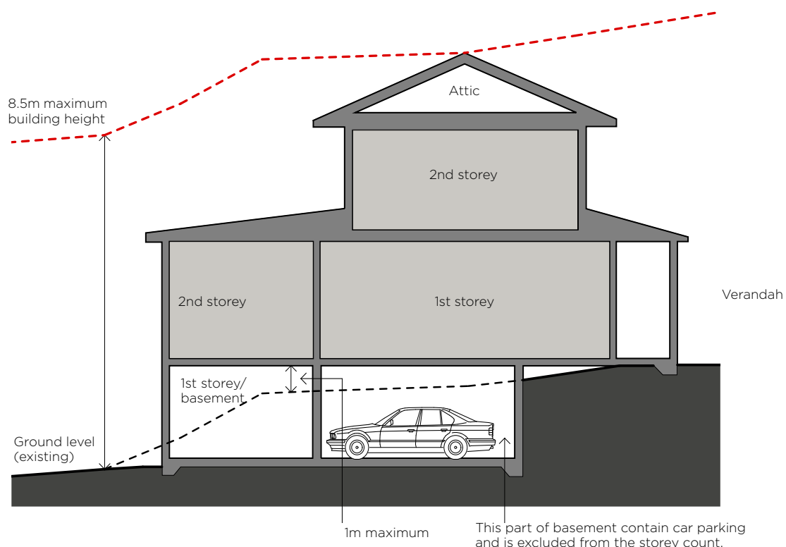
Figure 3-30 Calculating number of storeys
