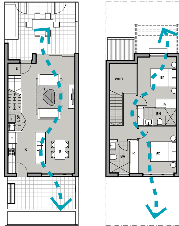
Figure 3-67 Cross ventilated dwelling
