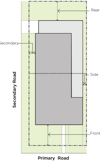
Figure 3-33 Nomination of setbacks for a corner dual occupancy
