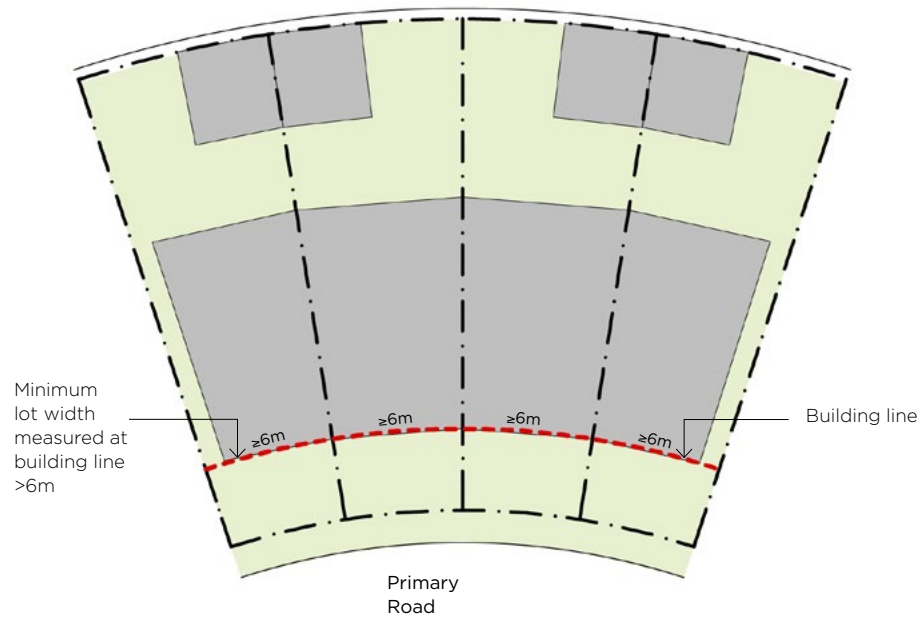
Figure 3-59 Street frontage width is measured at the building line for multi dwelling housing (terraces)
