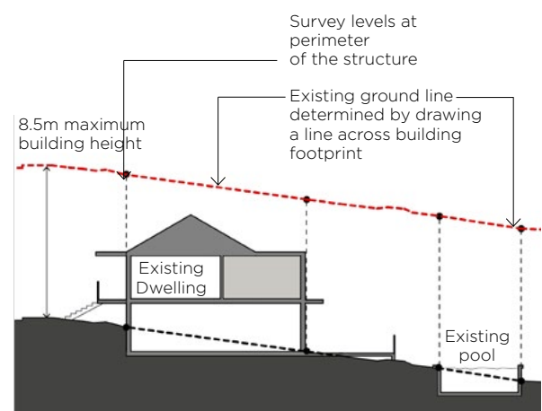
Figure 3-31 Determining existing ground level under existing structures
