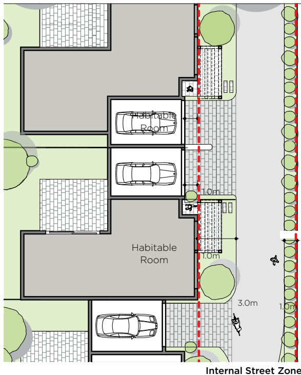
Figure 3-50 New internal lane providing access to dwellings behind street frontage and encouraging shared vehicle access arrangements
