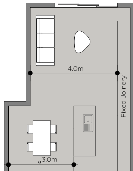
Figure 3-76 The minimum room dimension is the smallest dimension measured in any direction
