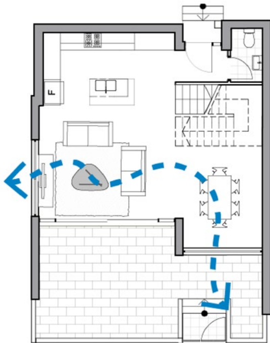
Figure 3-68 Corner cross ventilated dwelling
