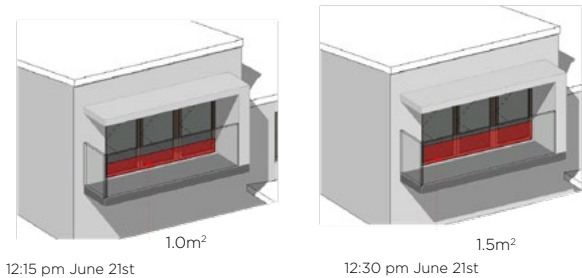
Figure 3-63 For solar access to be included, at least 1m 2 of sunlight must remain in a window for a 15 minute period
