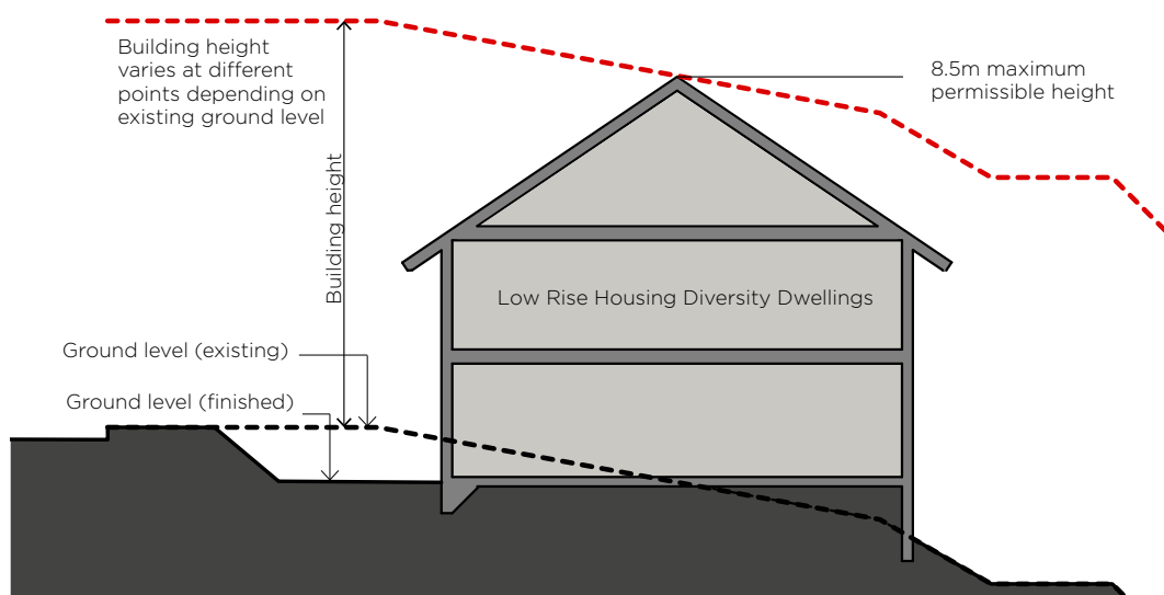
Figure 3-29 Measuring building height
