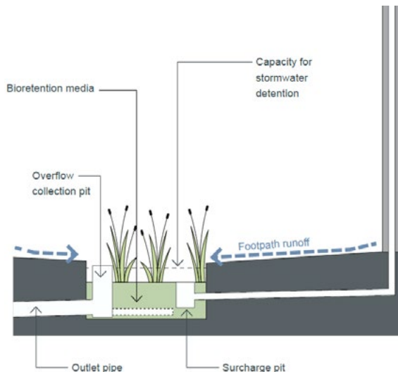
Figure 3-131 A bioretention garden improves water quality by using plants to treat roof and surface water runoff
