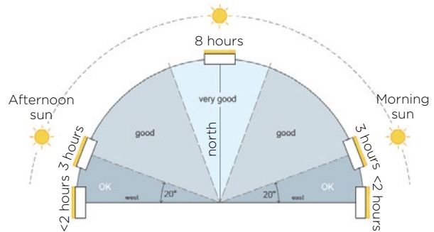
Figure 3-61 The hours of sunlight that can be expected in mid-winter are directly related to the orientation of the façade. This diagram shows the optimal orientation for habitable rooms and balconies
