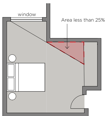
Figure 3-65 A window is visible from 75% of the floor area of a habitable room
