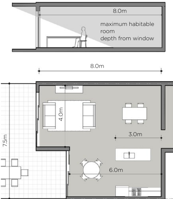
Figure 3-62 The depth of a single aspect dwelling relative to the ceiling height directly influences the quality of natural ventilation and daylight access. The maximum depth of open plan layouts combining living, dining and kitchen spaces is 8 metres.
