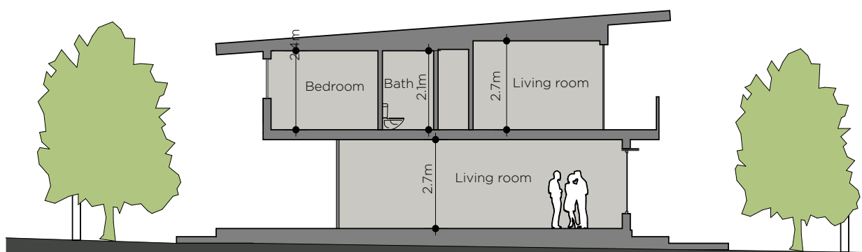
Figure 3-70 Different ceiling heights in different spaces
