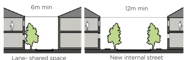
Figure 3-54 Minimum widths for shared lanes and internal streets
