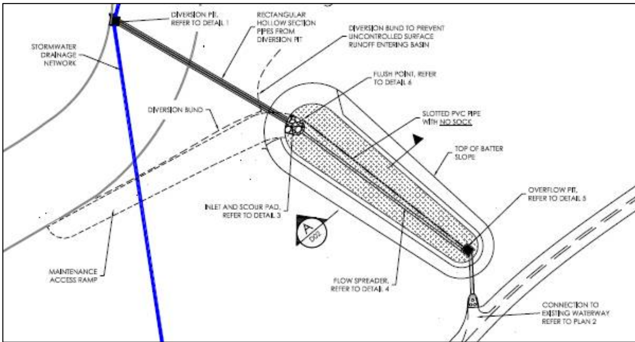
Figure 6-7 Typical Bioretention Layout – Flat Terrain
