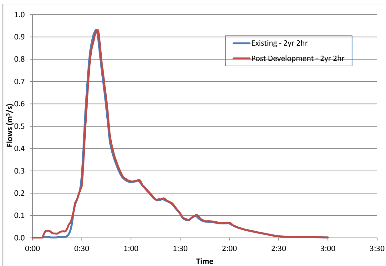
Figure A-7 Hydrograph Comparison at Flow Measurement Line L121
