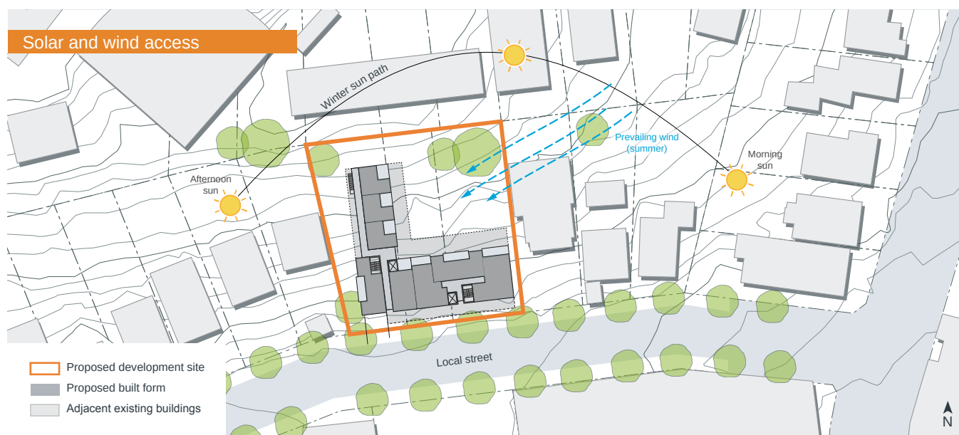
Figure 3A.4 Analysis of solar and wind access
