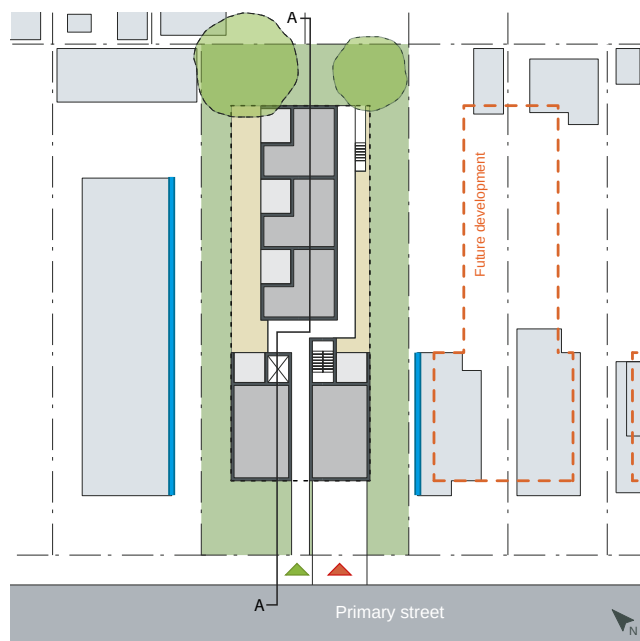
Proposed development - Typical ground level plan
