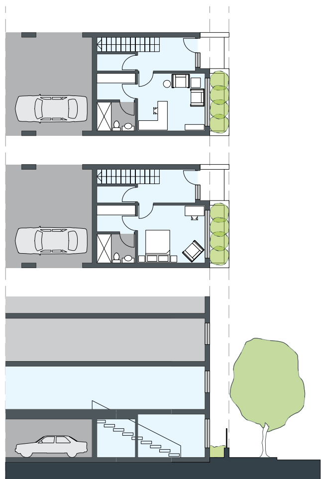
Figure 3J.17 Above ground parking should be concealed behind the building facade and wrapped with other uses along the primary street frontage, such as retail, commercial or two storey SOHO units
